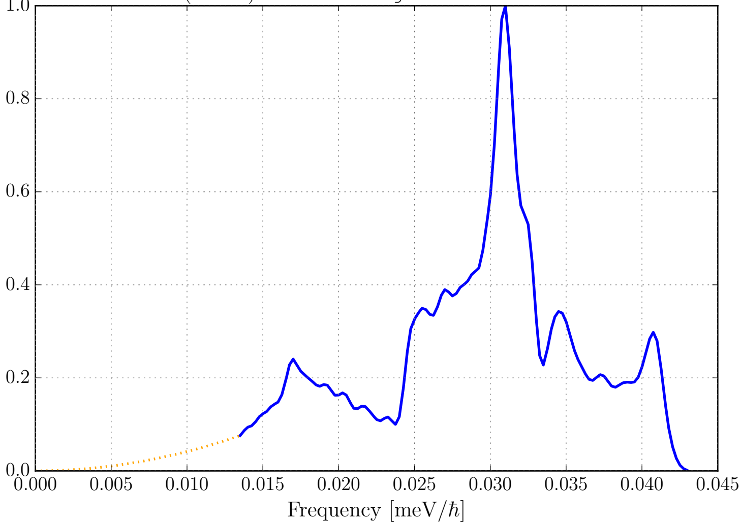
Phonon DOS (VDOS) for F in NaF_sg225_SodiumFlouride.ncmat
