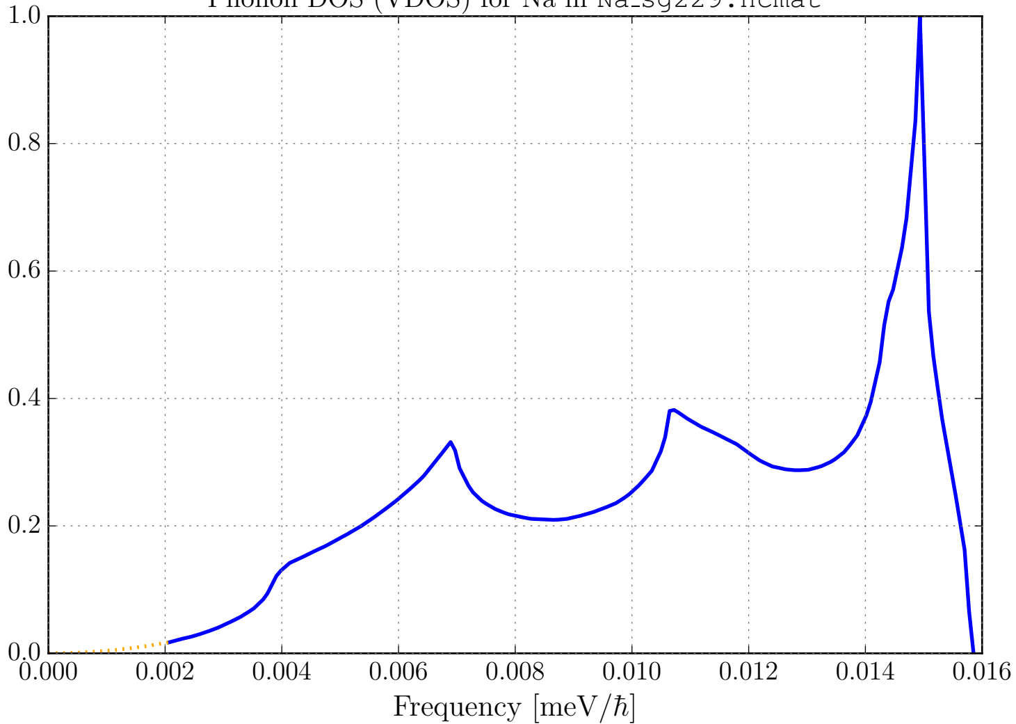
Phonon DOS (VDOS) for Na in Na_sg229.ncmat
