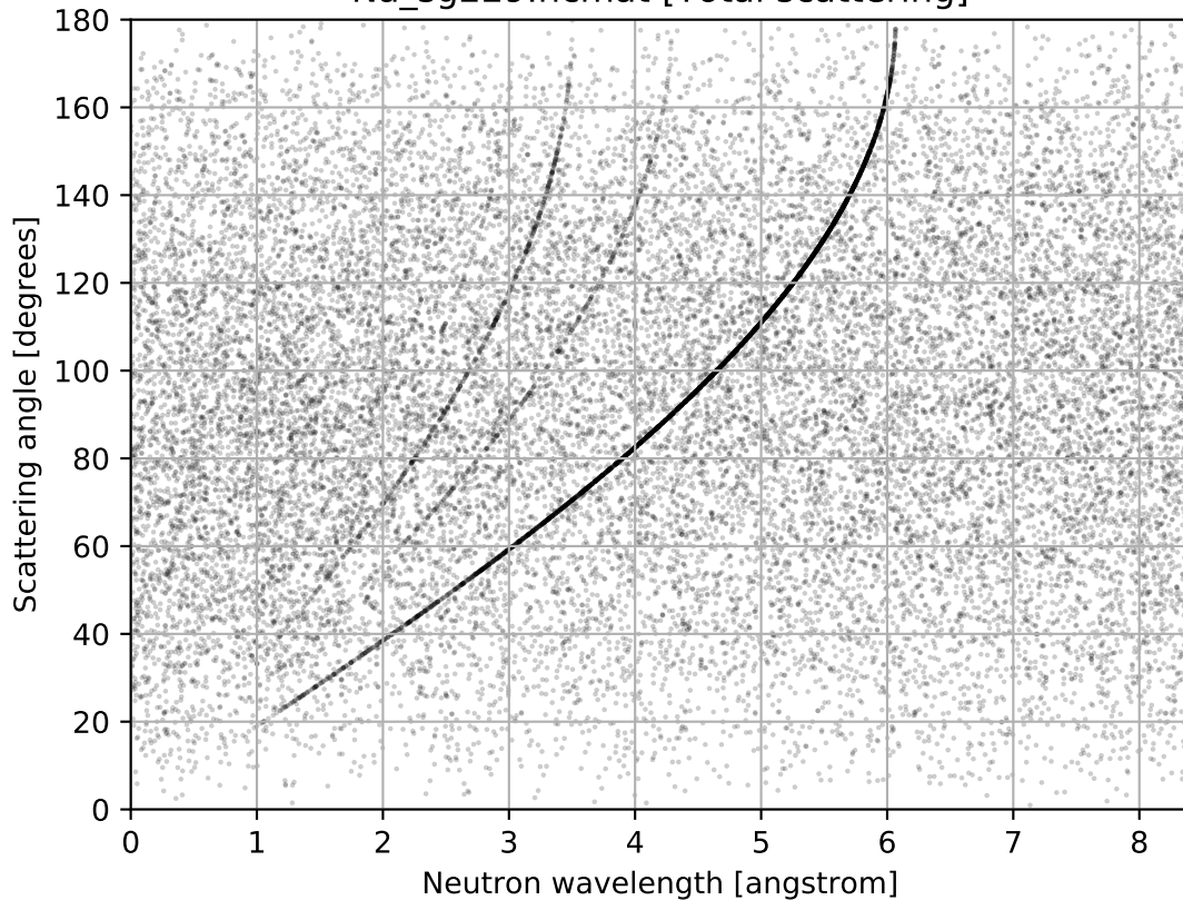
Na_sg229.ncmat [Total scattering]
