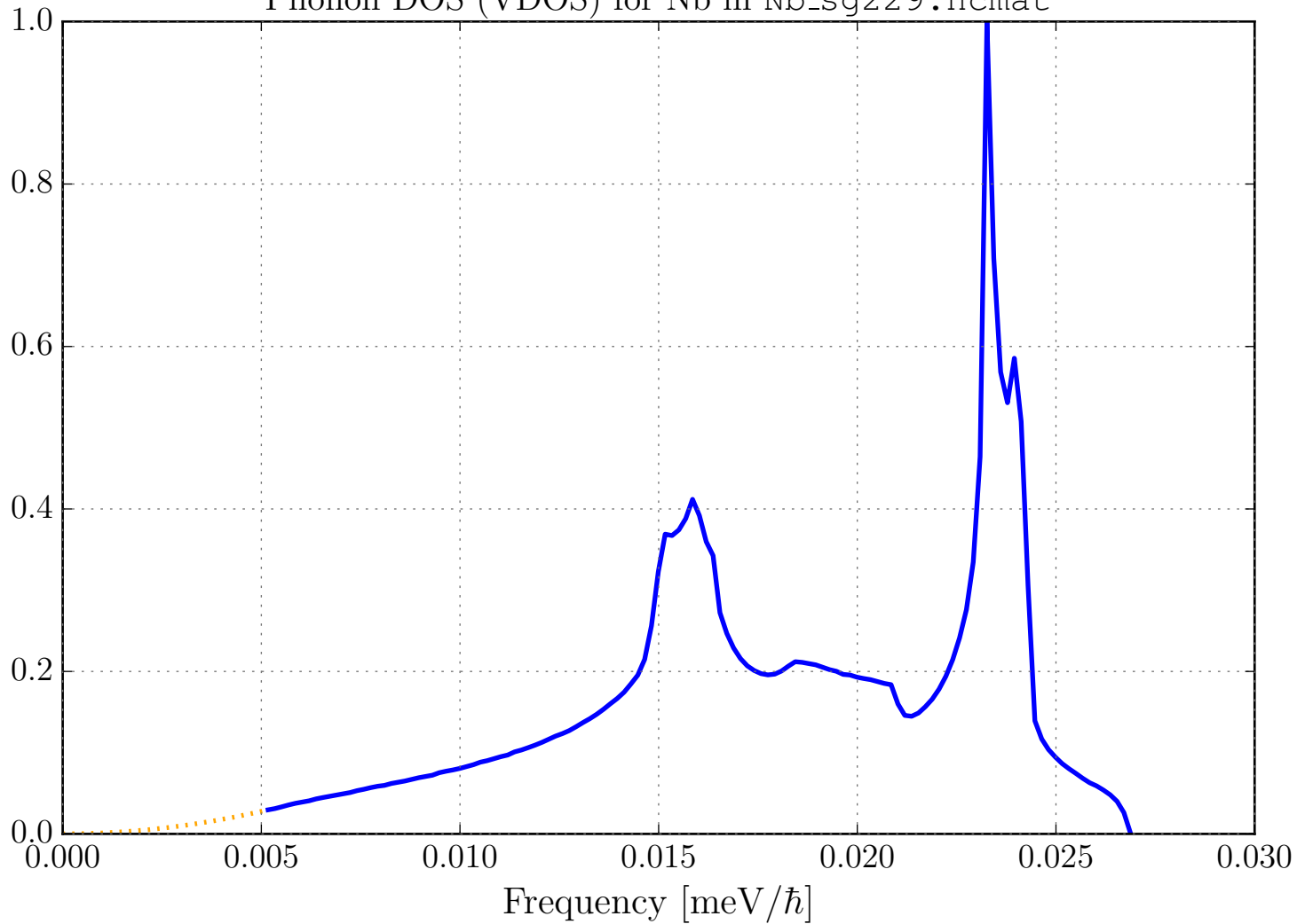
Phonon DOS (VDOS) for Nb in Nb_sg229.ncmat
