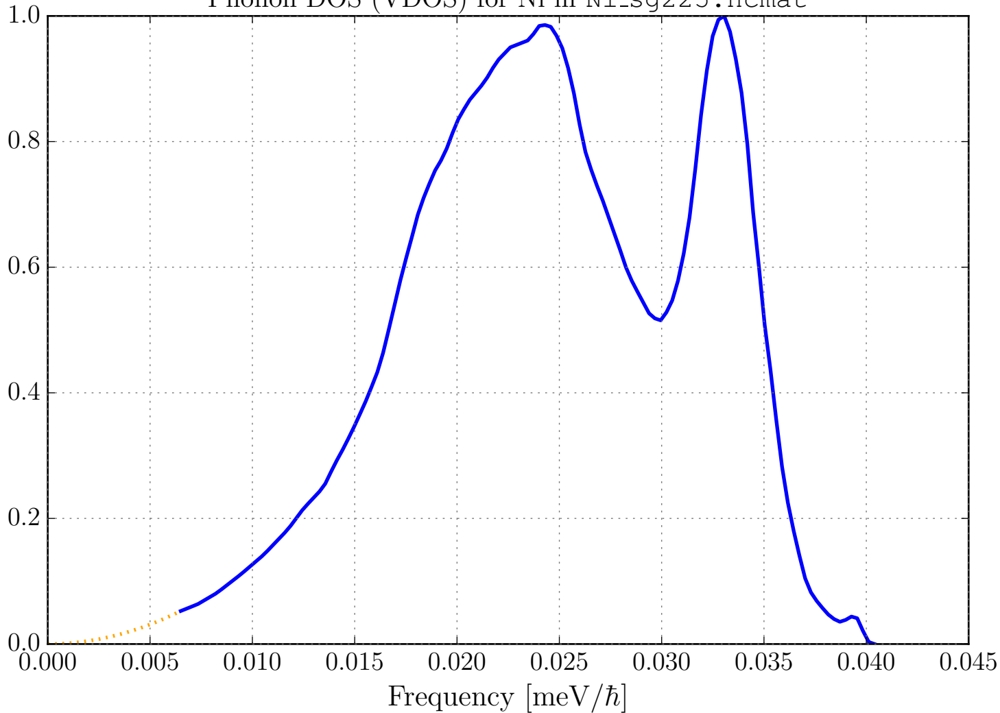
Phonon DOS (VDOS) for Ni in Ni_sg225.ncmat
