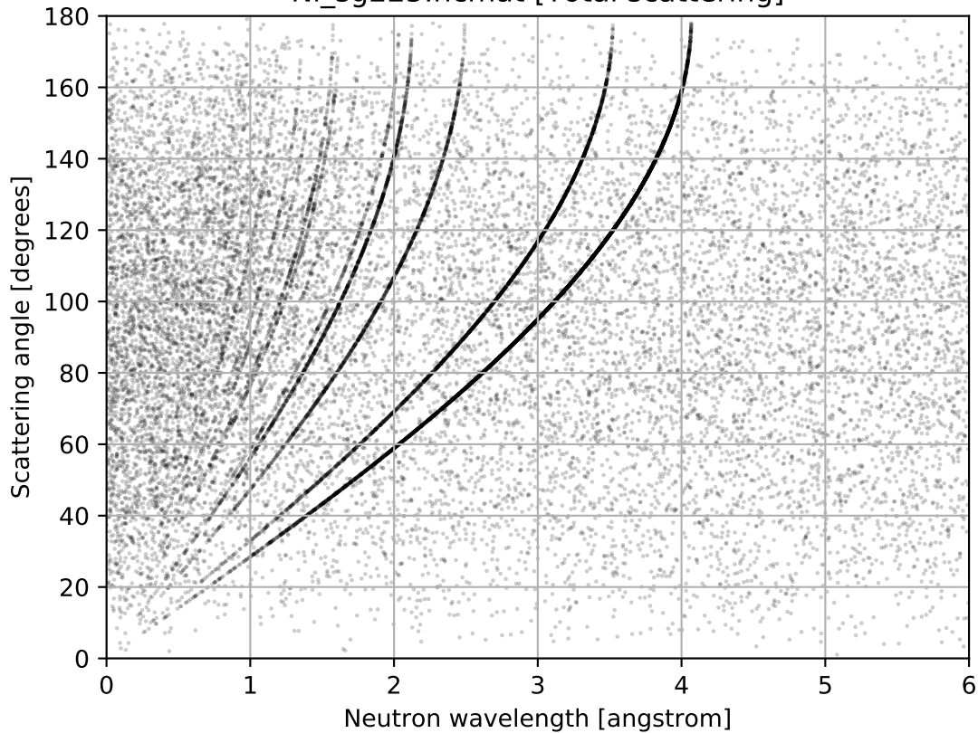
Ni_sg225.ncmat [Total scattering]
