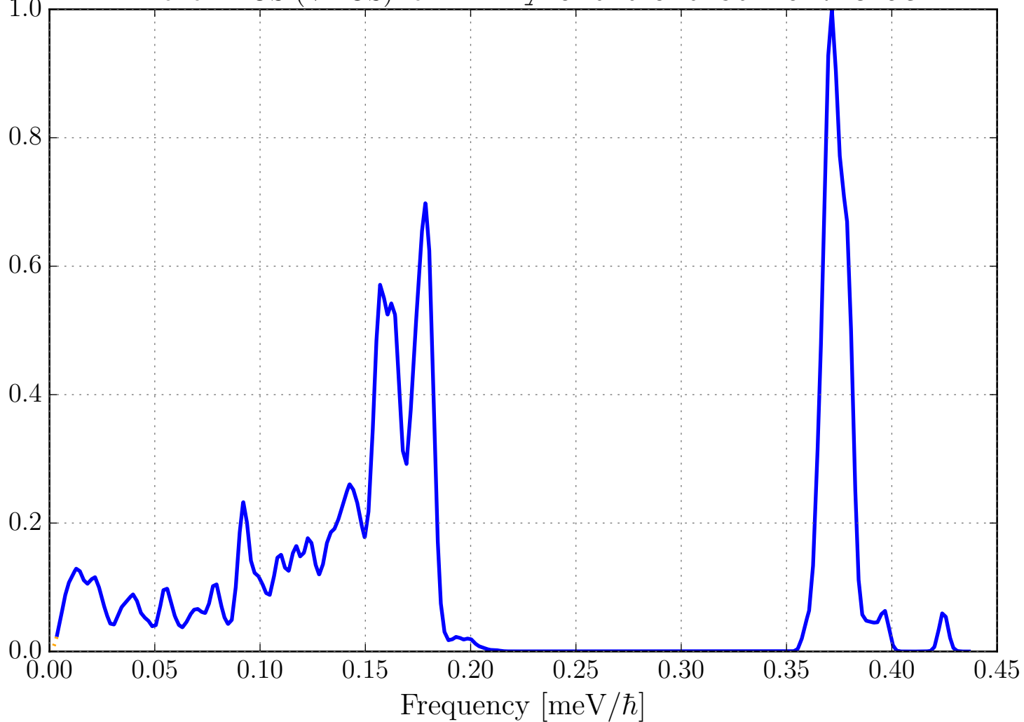
Phonon DOS (VDOS) for H in Nylon610_C16H30N2O2.ncmat
