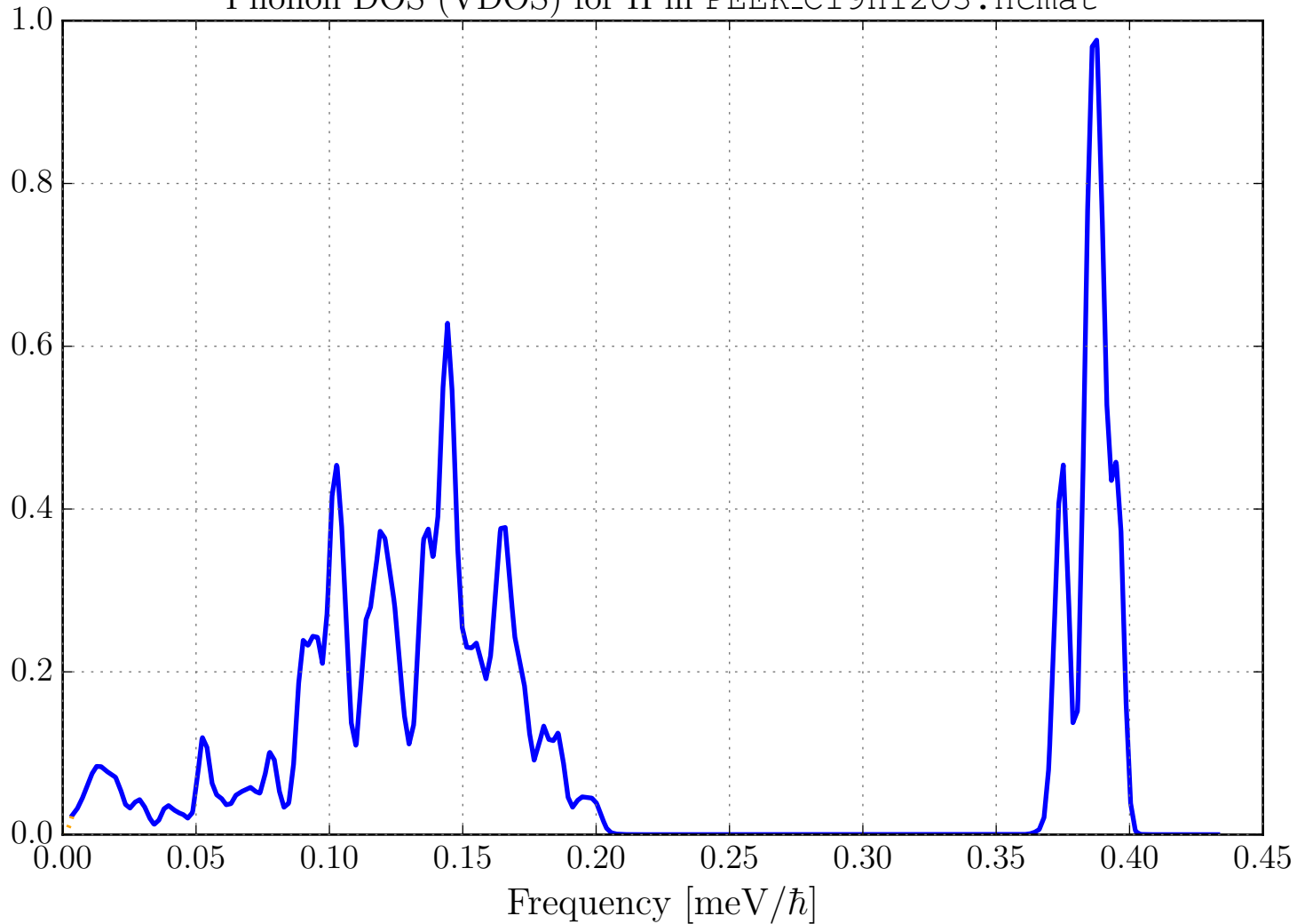
Phonon DOS (VDOS) for H in PEEK_C19H12O3.ncmat
