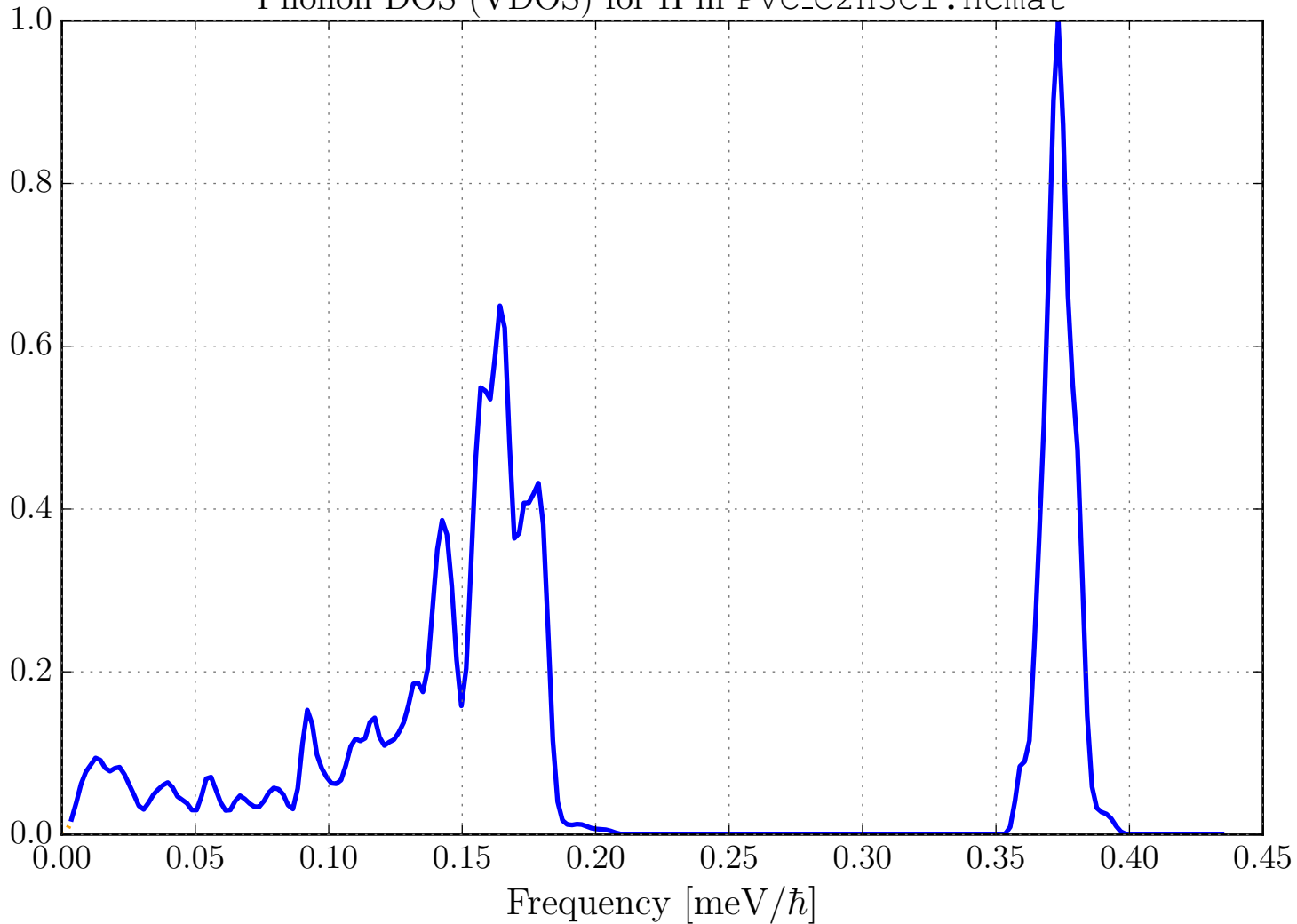
Phonon DOS (VDOS) for H in PVC_C2H3Cl.ncmat
