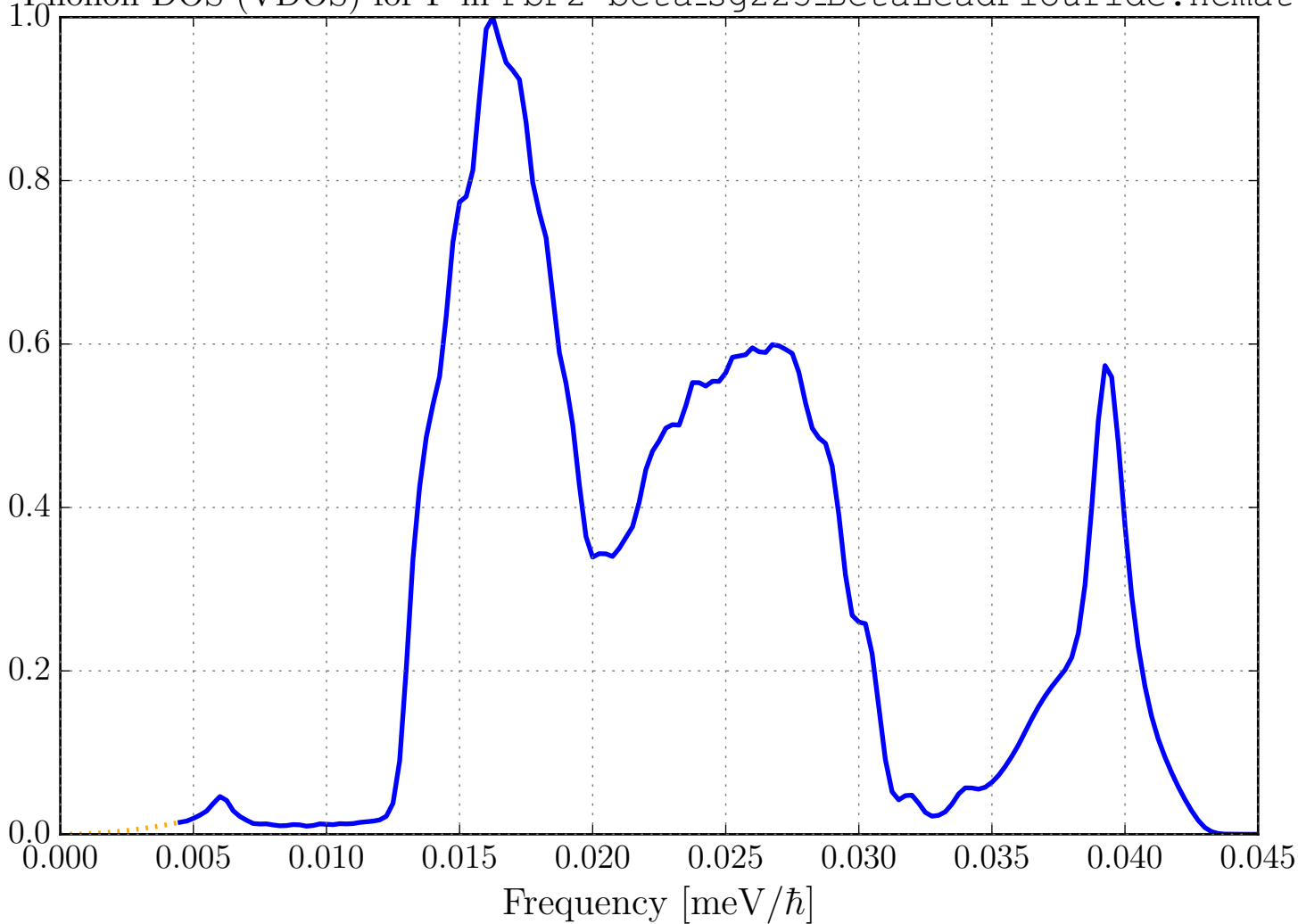
Phonon DOS (VDOS) for F in PbF2-beta_sg225_BetaLeadFlouride.ncmat
