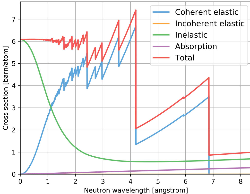
PbF2-beta_sg225_BetaLeadFlouride.ncmat
