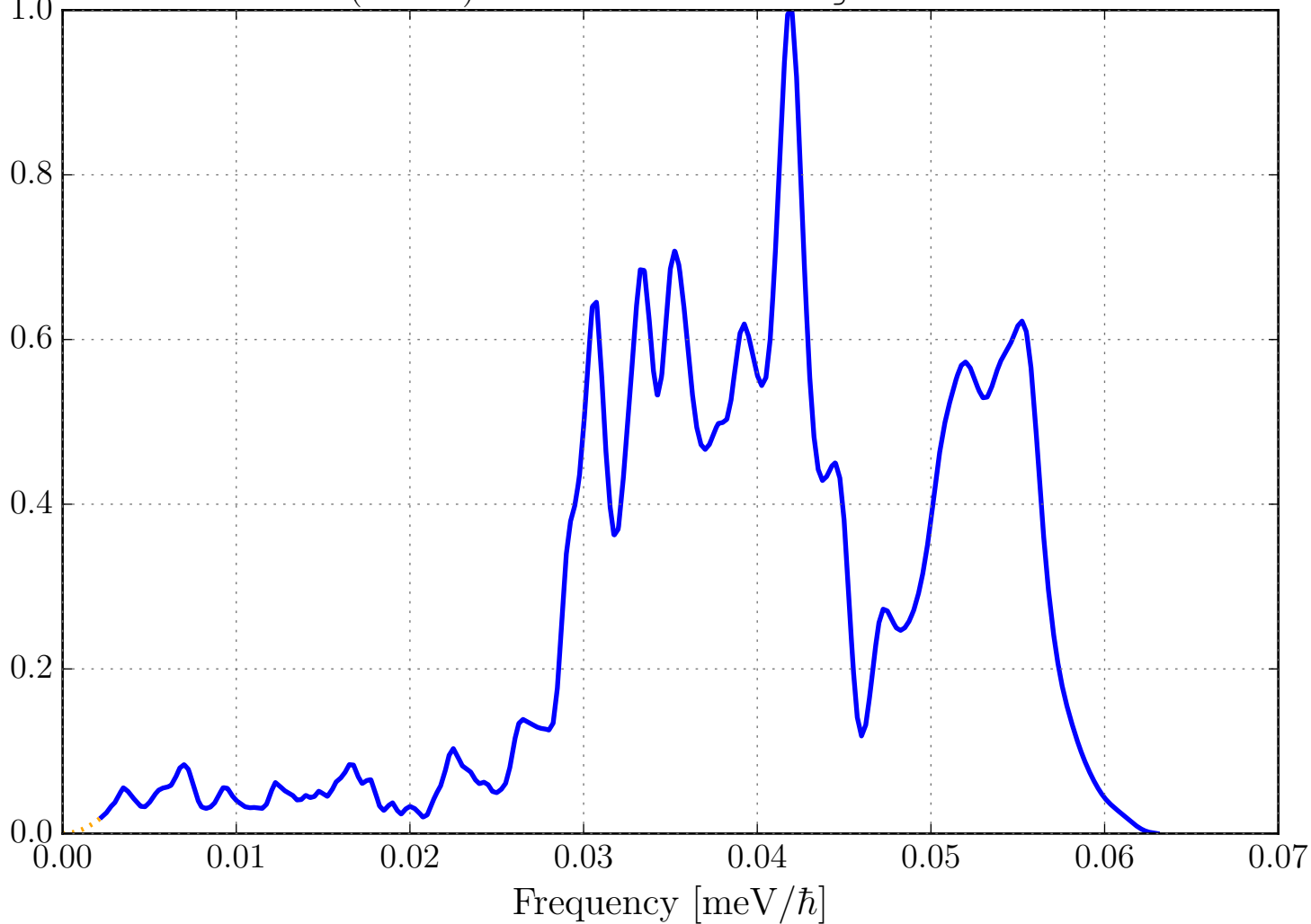
Phonon DOS (VDOS) for O in PbO-beta_sg57_Massicot.ncmat
