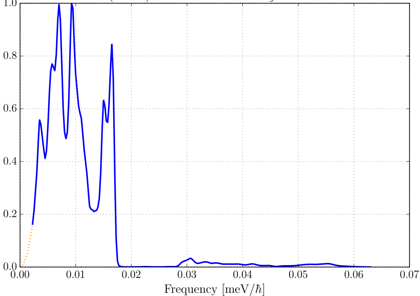
Phonon DOS (VDOS) for Pb in PbO-beta_sg57_Massicot.ncmat
