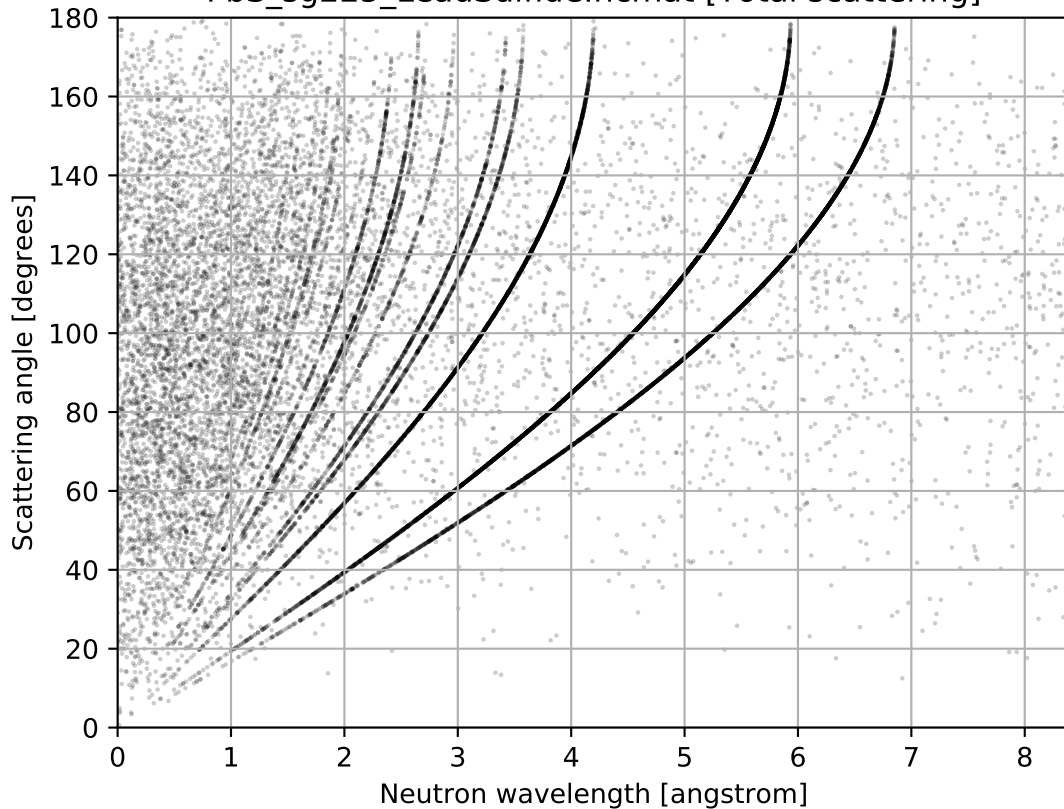
PbS_sg225_LeadSulfide.ncmat [Total scattering]
