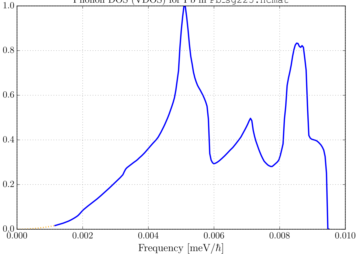
Phonon DOS (VDOS) for Pb in Pb_sg225.ncmat
