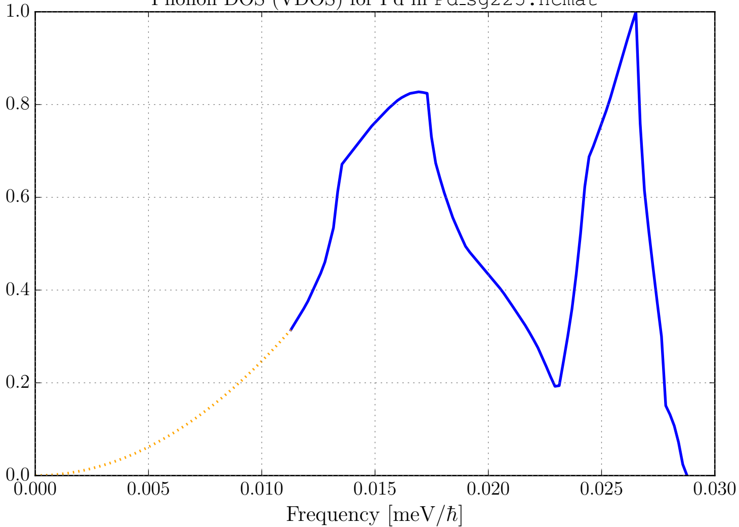
Phonon DOS (VDOS) for Pd in Pd_sg225.ncmat
