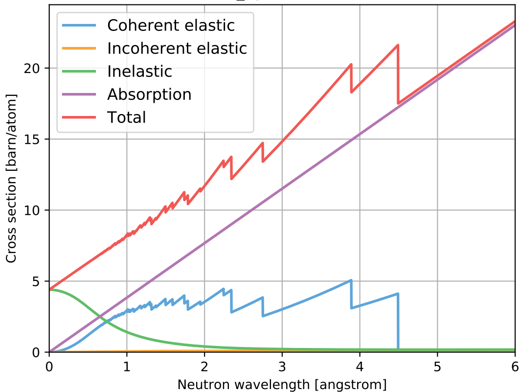
Pd_sg225.ncmat
