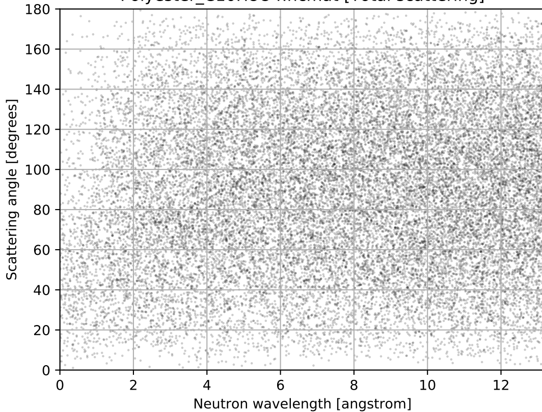
Polyester_C10H8O4.ncmat [Total scattering]
