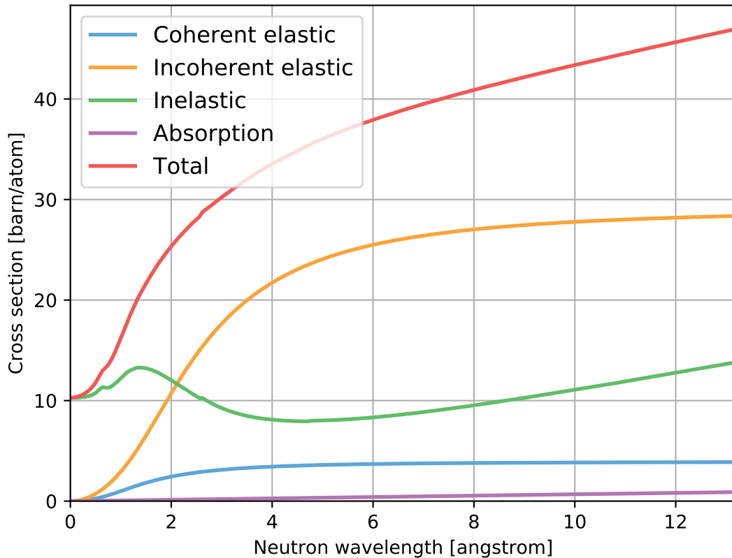
Polyester_C10H8O4.ncmat
