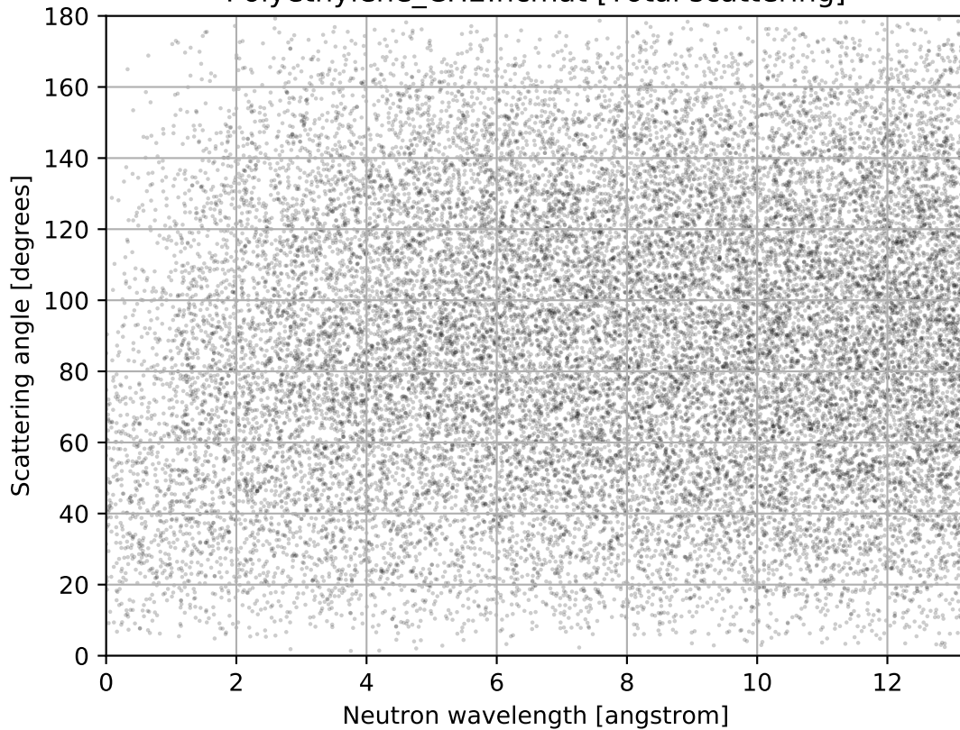
Polyethylene_CH2.ncmat [Total scattering]
