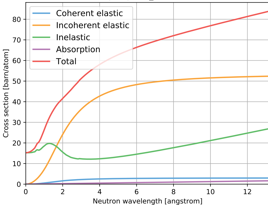
Polyethylene_CH2.ncmat
