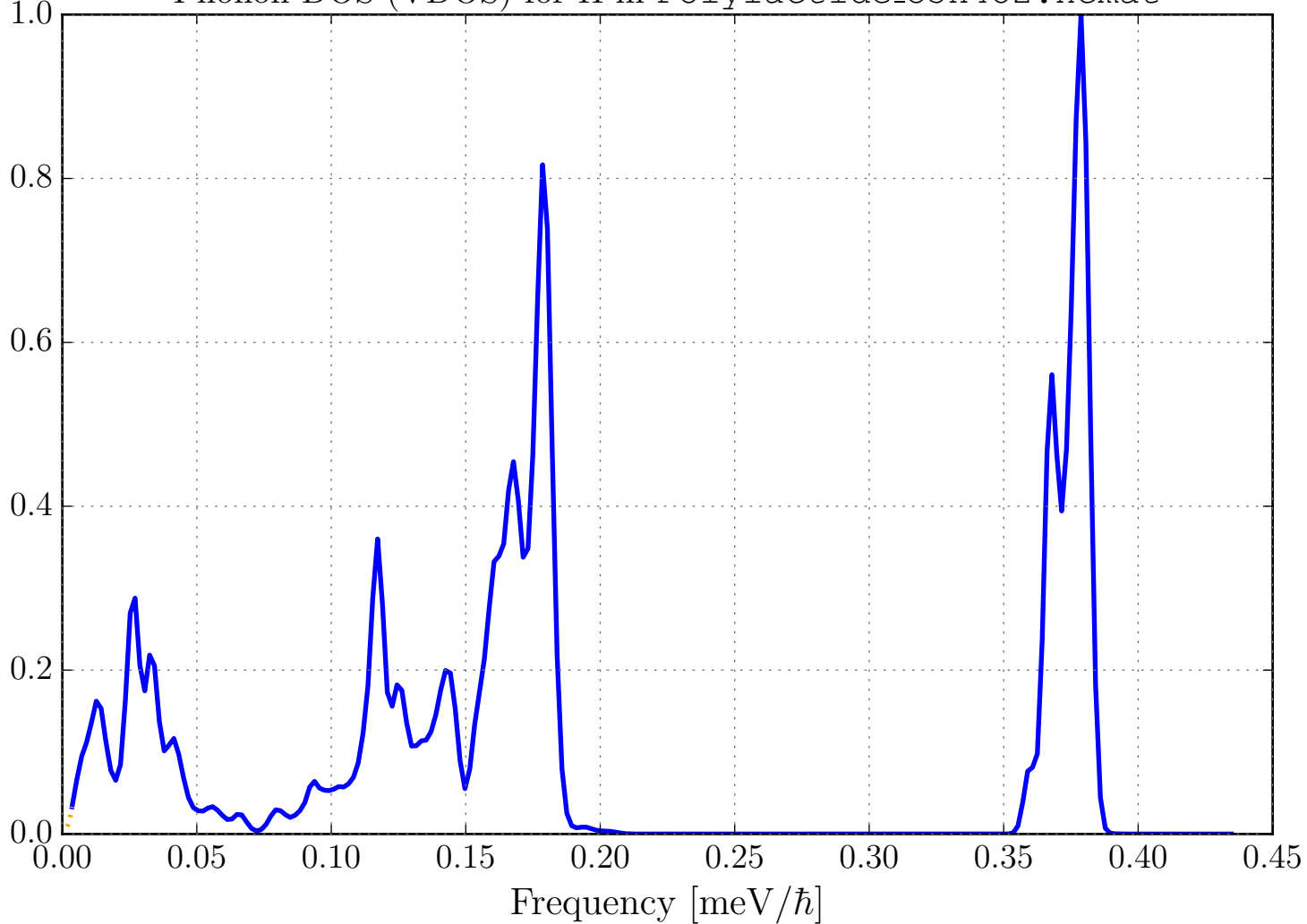
Phonon DOS (VDOS) for H in Poly lactide_C3H4O2.ncmat
