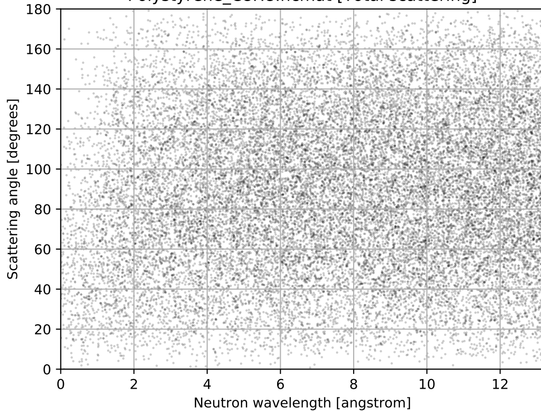
Polystyrene_C8H8.ncmat [Total scattering]
