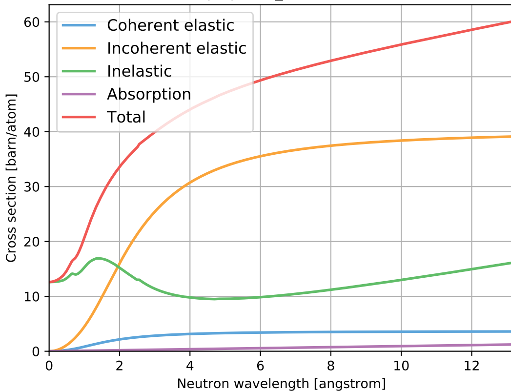
Polystyrene_C8H8.ncmat
