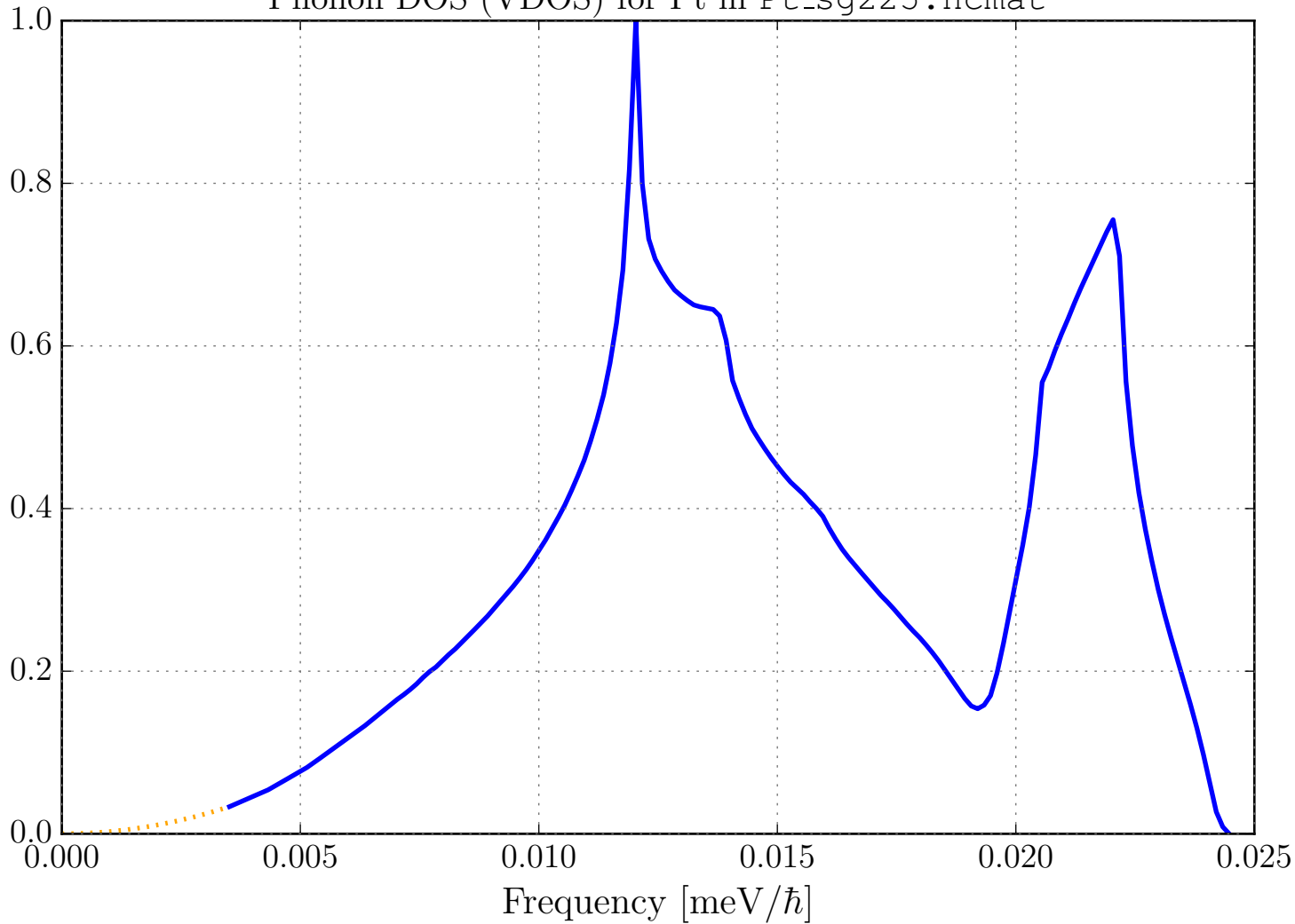
Phonon DOS (VDOS) for Pt in Pt_sg225.ncmat
