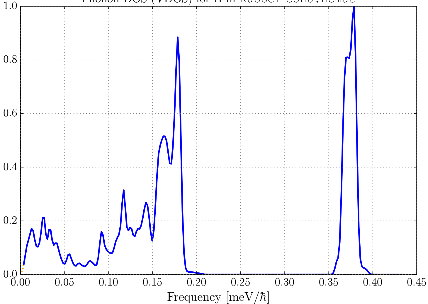
Phonon DOS (VDOS) for H in Rubber_C5H8.ncmat
