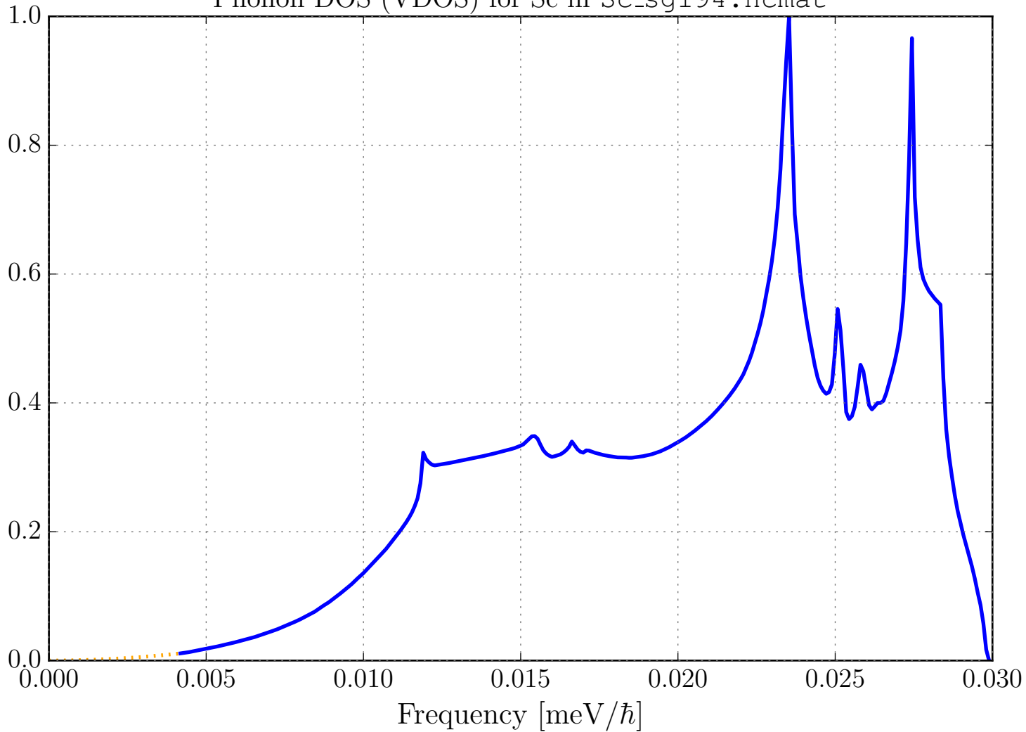
Phonon DOS (VDOS) for Sc in Sc_sg194.ncmat
