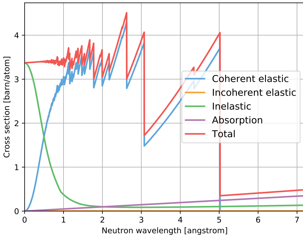
SiC-beta_sg216_BetaSiliconCarbide.ncmat
