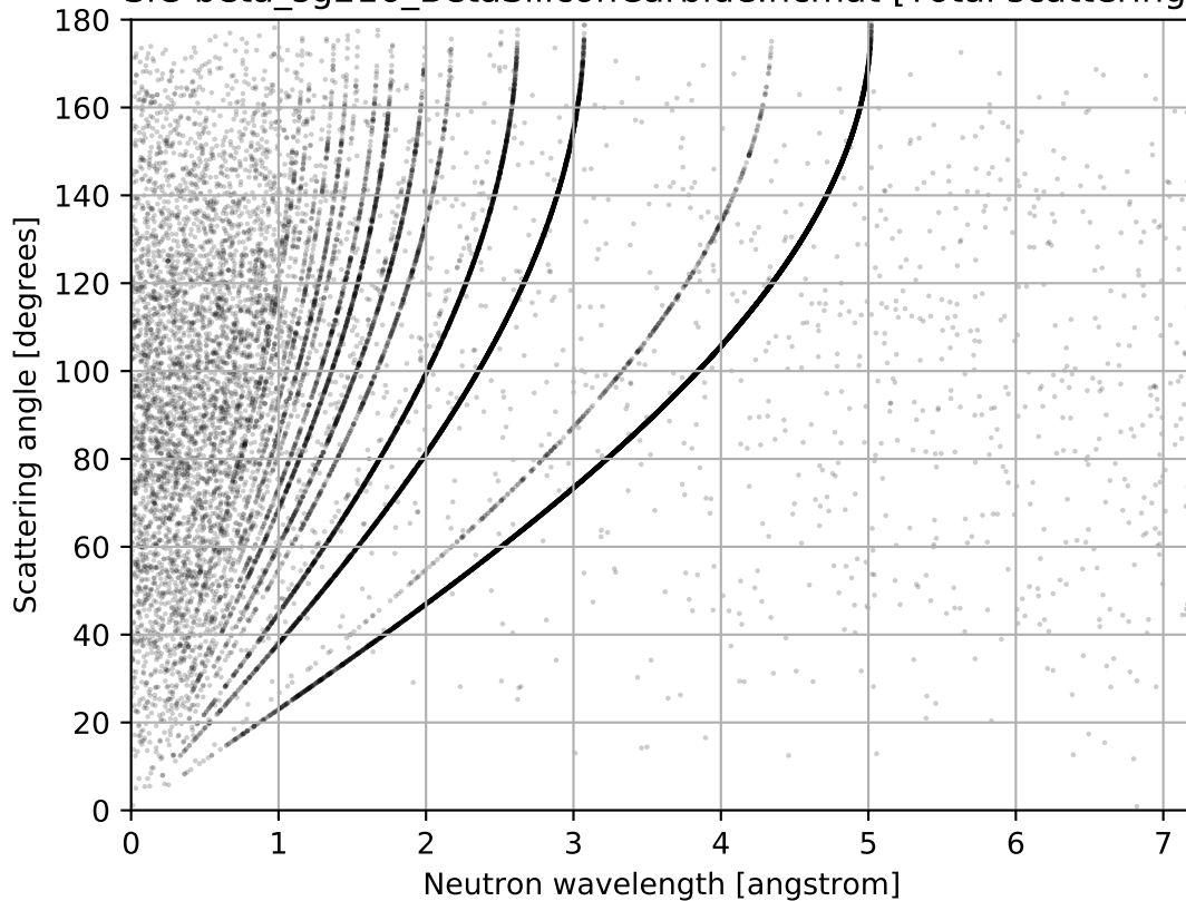
SiC-beta_sg216_BetaSiliconCarbide.ncmat [Total scattering]
