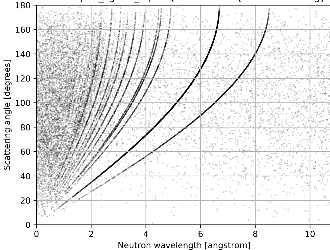
SiO2-alpha_sg154_AlphaQuartz.ncmat [Total scattering]
