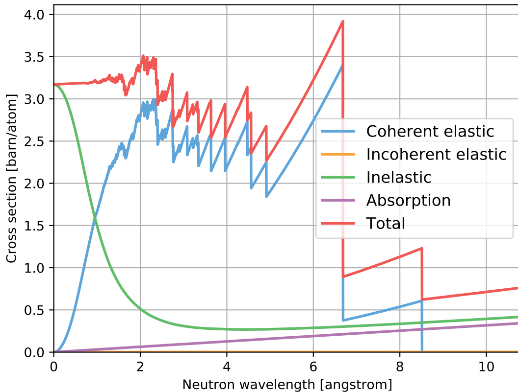
SiO2-alpha_sg154_AlphaQuartz.ncmat
