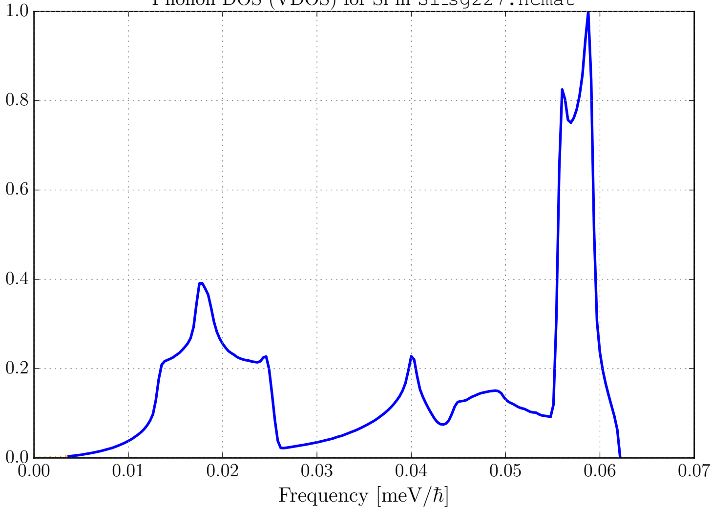
Phonon DOS (VDOS) for Si in Si_sg227.ncmat
