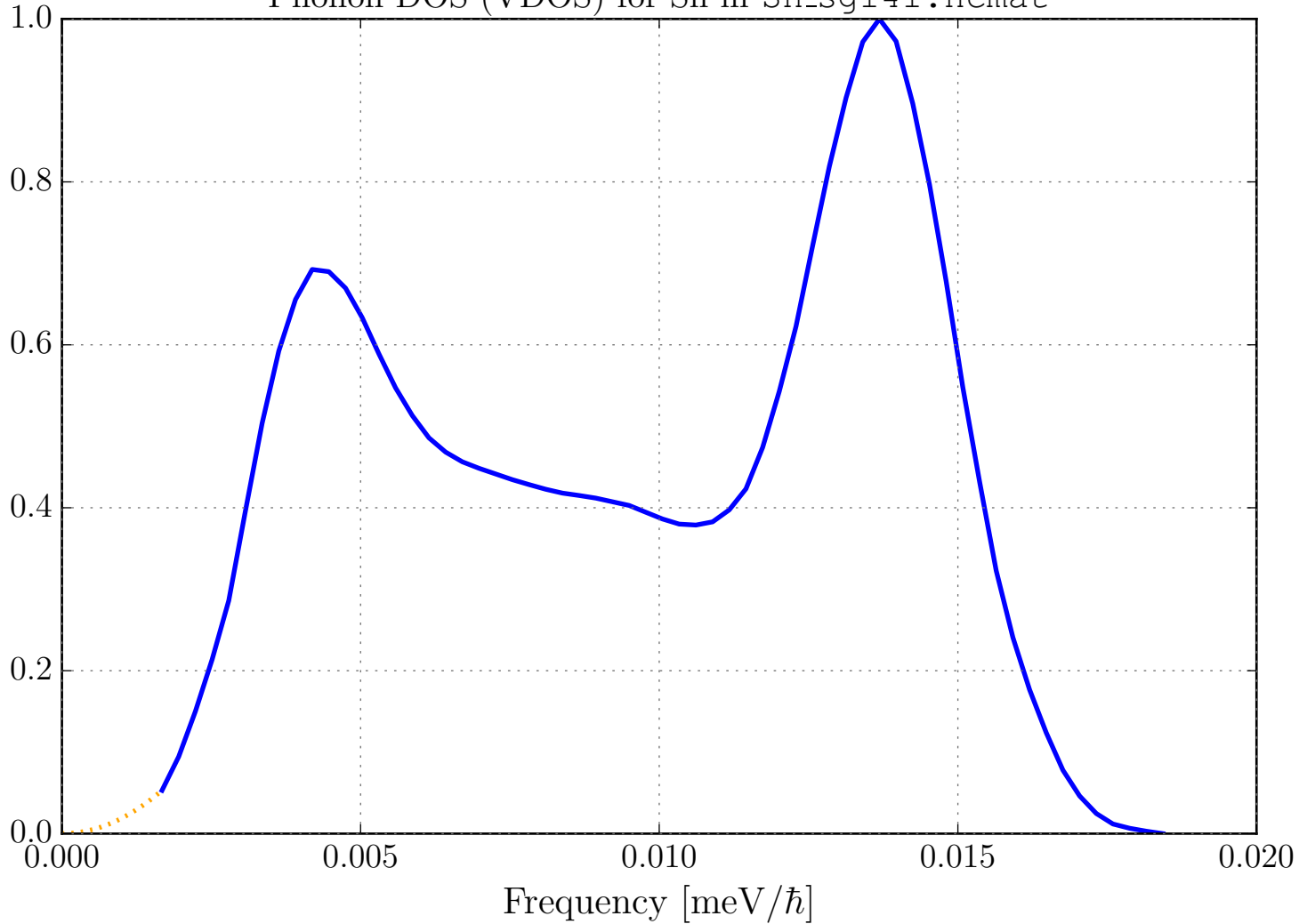
Phonon DOS (VDOS) for Sn in Sn_sg141.ncmat
