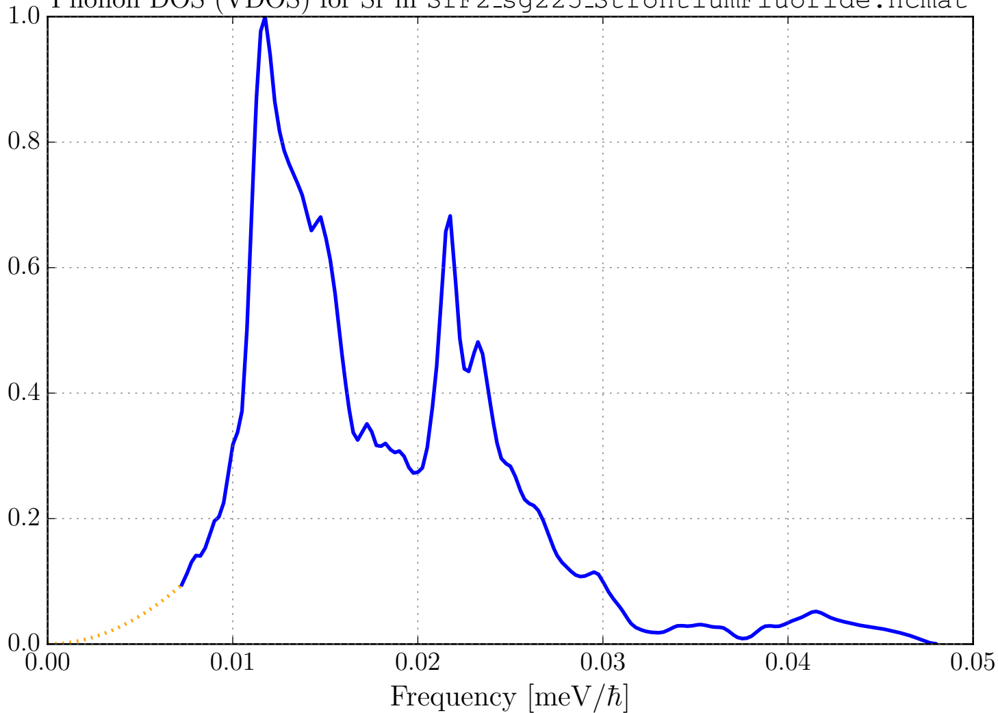
Phonon DOS (VDOS) for Sr in SrF2_sg225_StrontiumFluoride.ncmat
