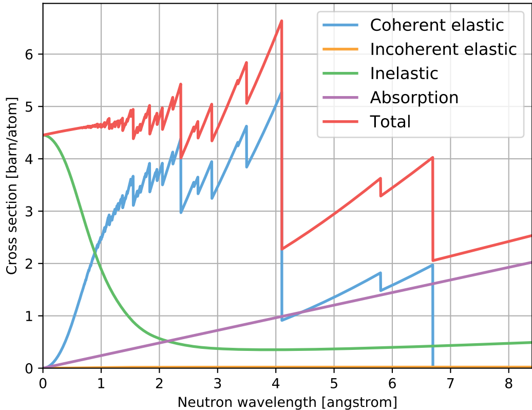
SrF2_sg225_StrontiumFluoride.ncmat
