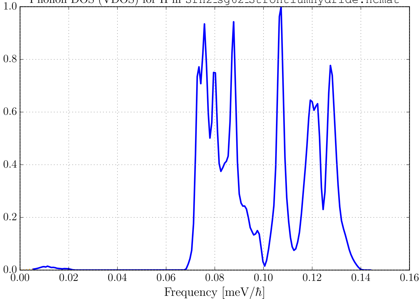
Phonon DOS (VDOS) for H in SrH2_sg62_StrontiumHydride.ncmat
