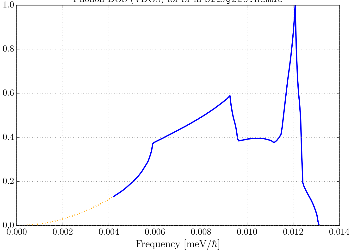
Phonon DOS (VDOS) for Sr in Sr_sg225.ncmat
