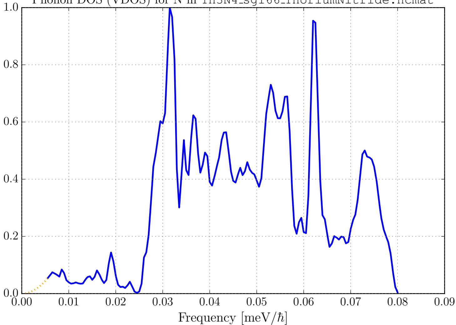
Phonon DOS (VDOS) for N in Th3N4_sg166_ThoriumNitride.ncmat
