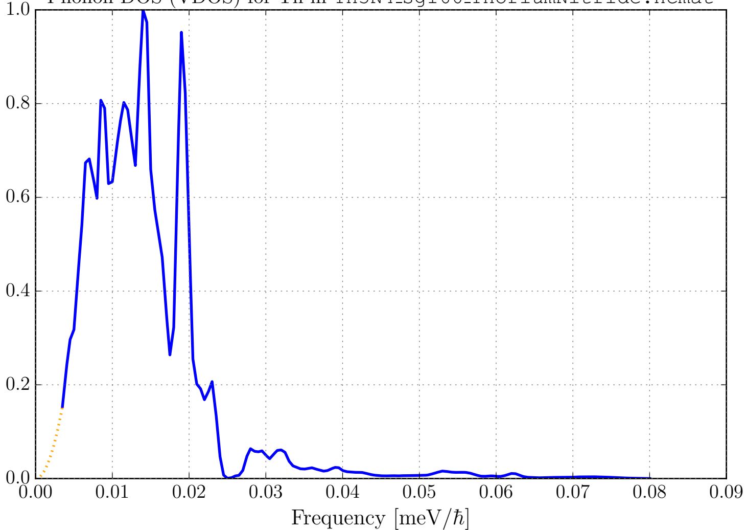
Phonon DOS (VDOS) for Th in Th3N4_sg166_ThoriumNitride.ncmat
