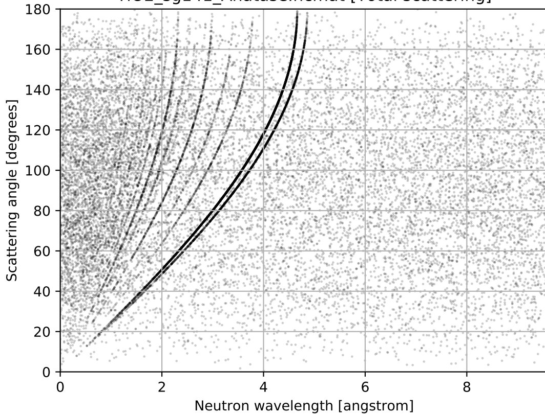
TiO2_sg141_Anatase.ncmat [Total scattering]
