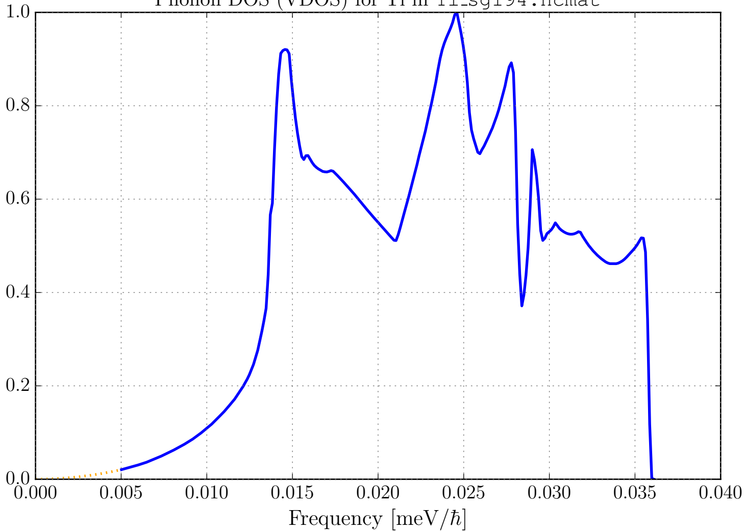
Phonon DOS (VDOS) for Ti in Ti_sg194.ncmat
