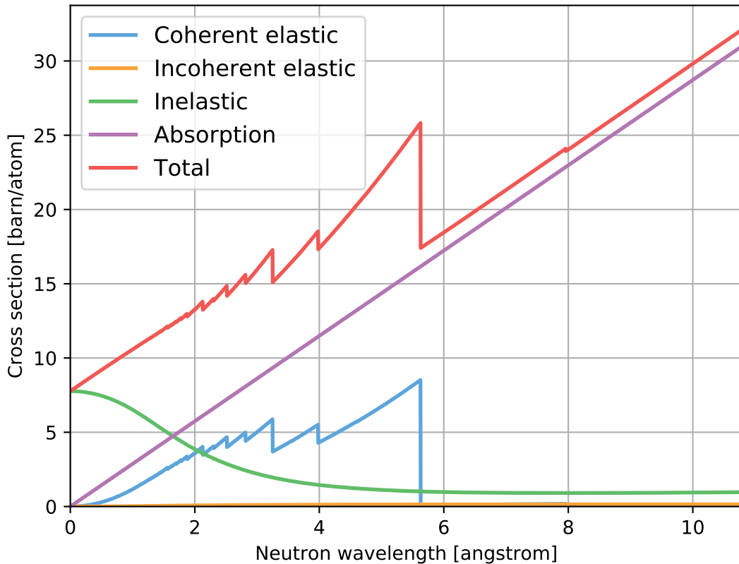
TlBr_sg221_ThaliumBromide.ncmat
