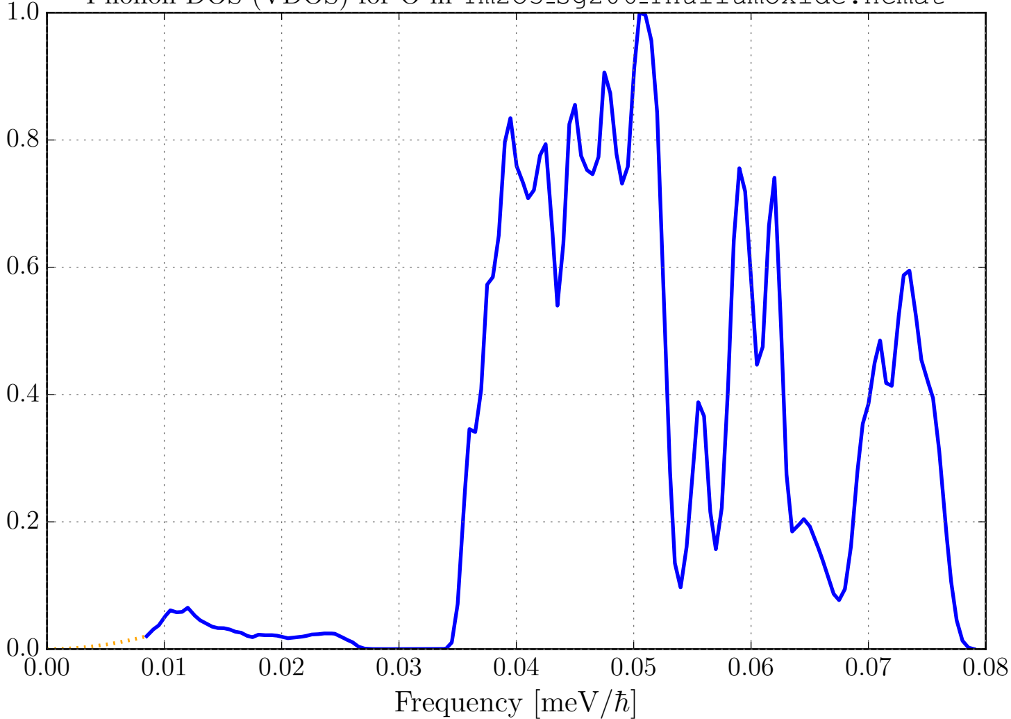
Phonon DOS (VDOS) for O in Tm2O3_sg206_ThuliumOxide.ncmat
