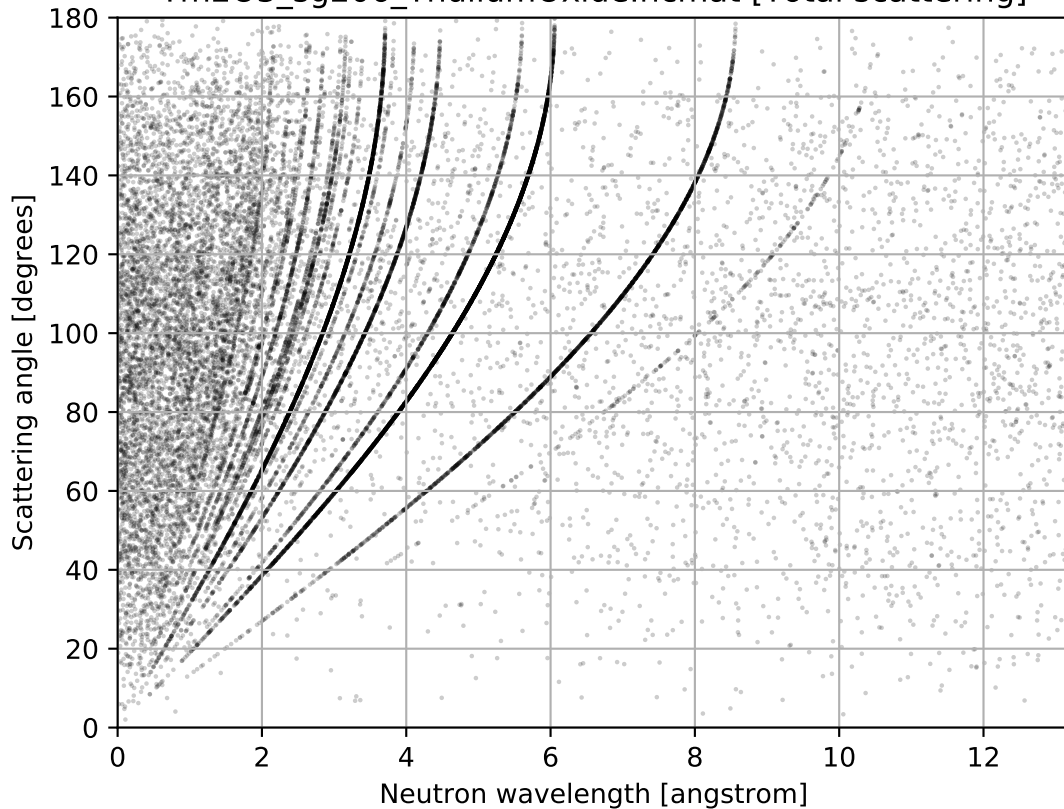
Tm2O3_sg206_ThuliumOxide.ncmat [Total scattering]
