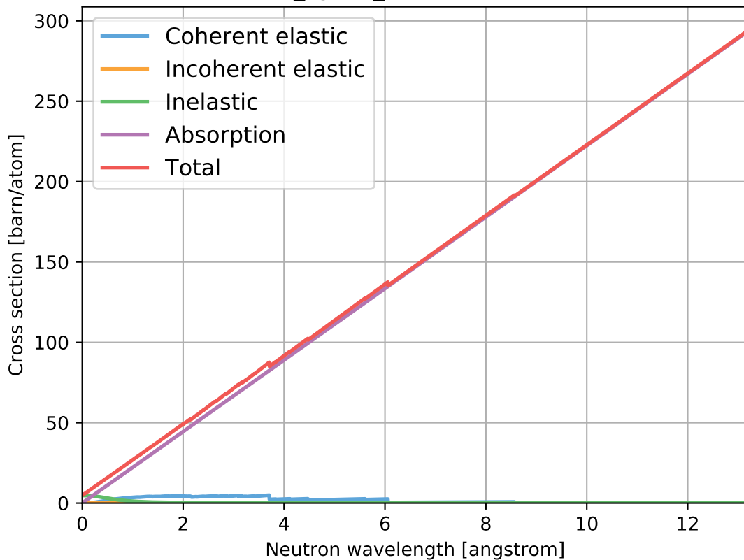
Tm2O3_sg206_ThuliumOxide.ncmat
