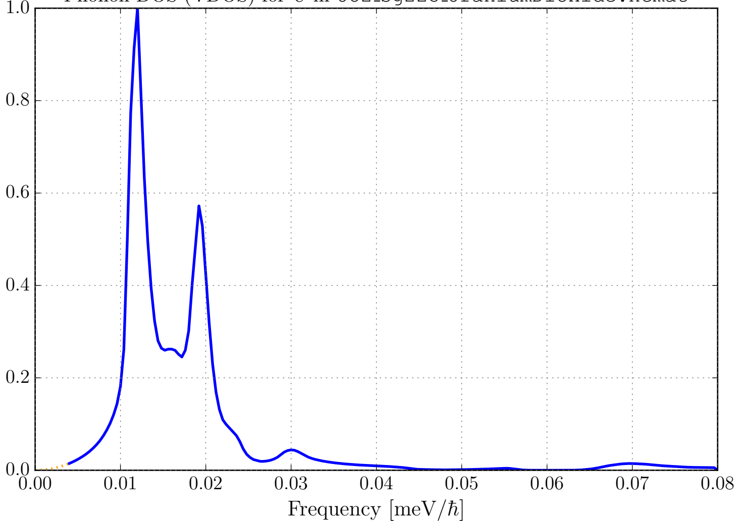
Phonon DOS (VDOS) for U in UO2_sg225-UraniumDioxide.ncmat
