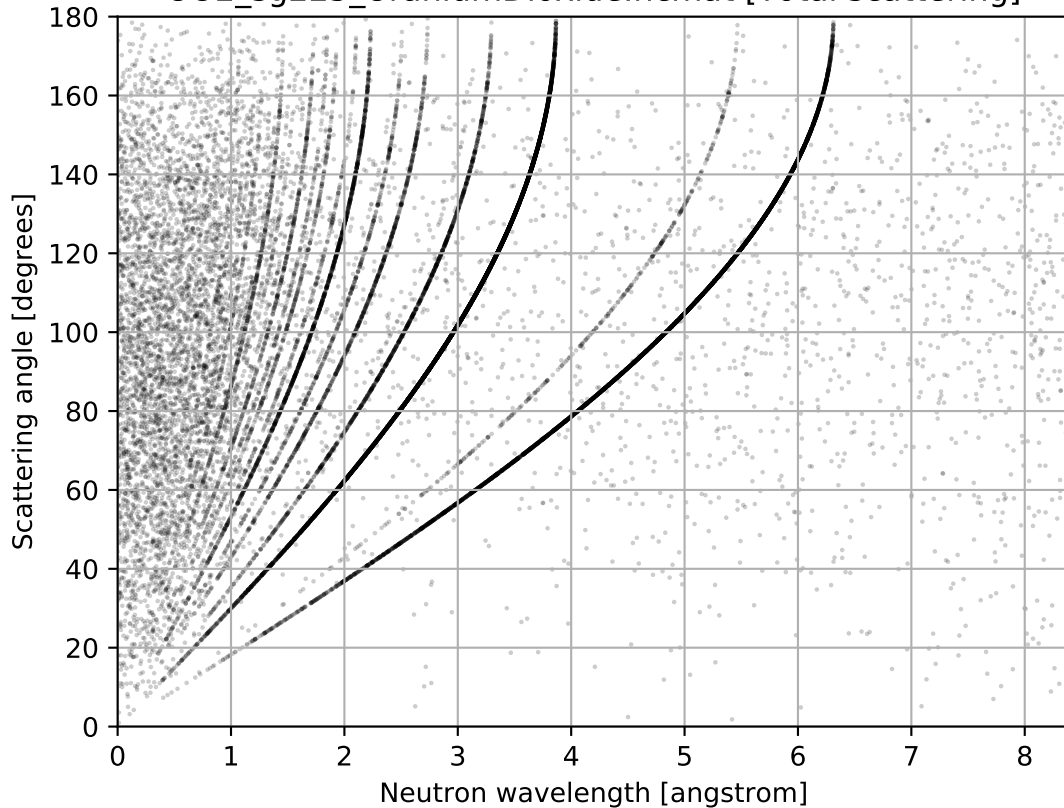
UO2_sg225_UraniumDioxide.ncmat [Total scattering]
