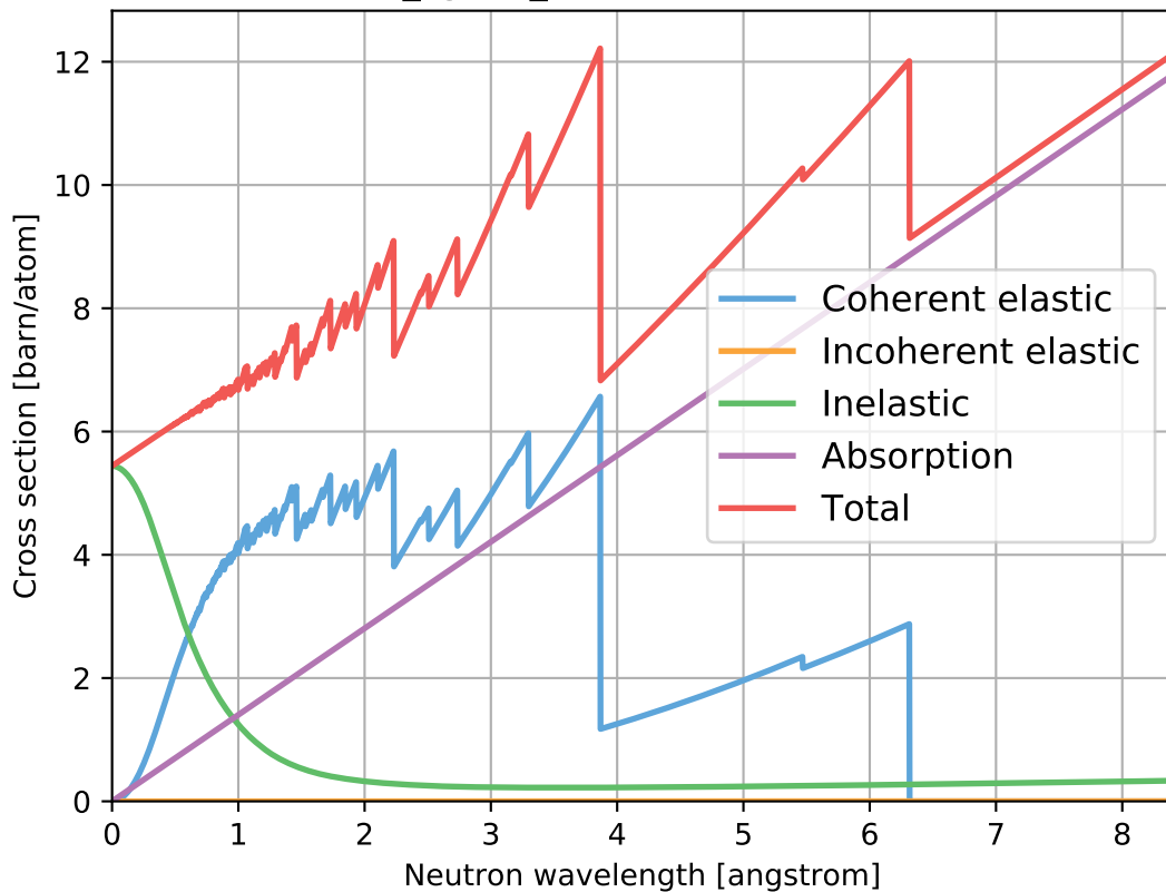
UO2_sg225_UraniumDioxide.ncmat
