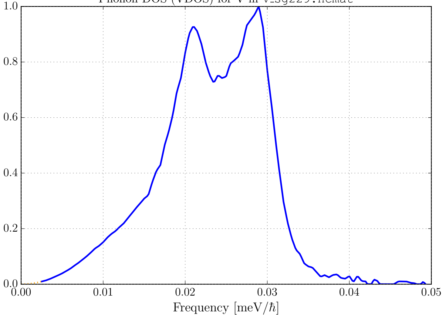
Phonon DOS (VDOS) for V in V_sg229.ncmat
