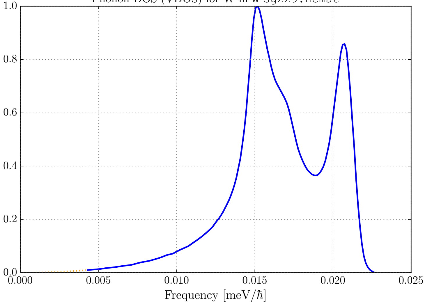
Phonon DOS (VDOS) for W in w_sg229.ncmat
