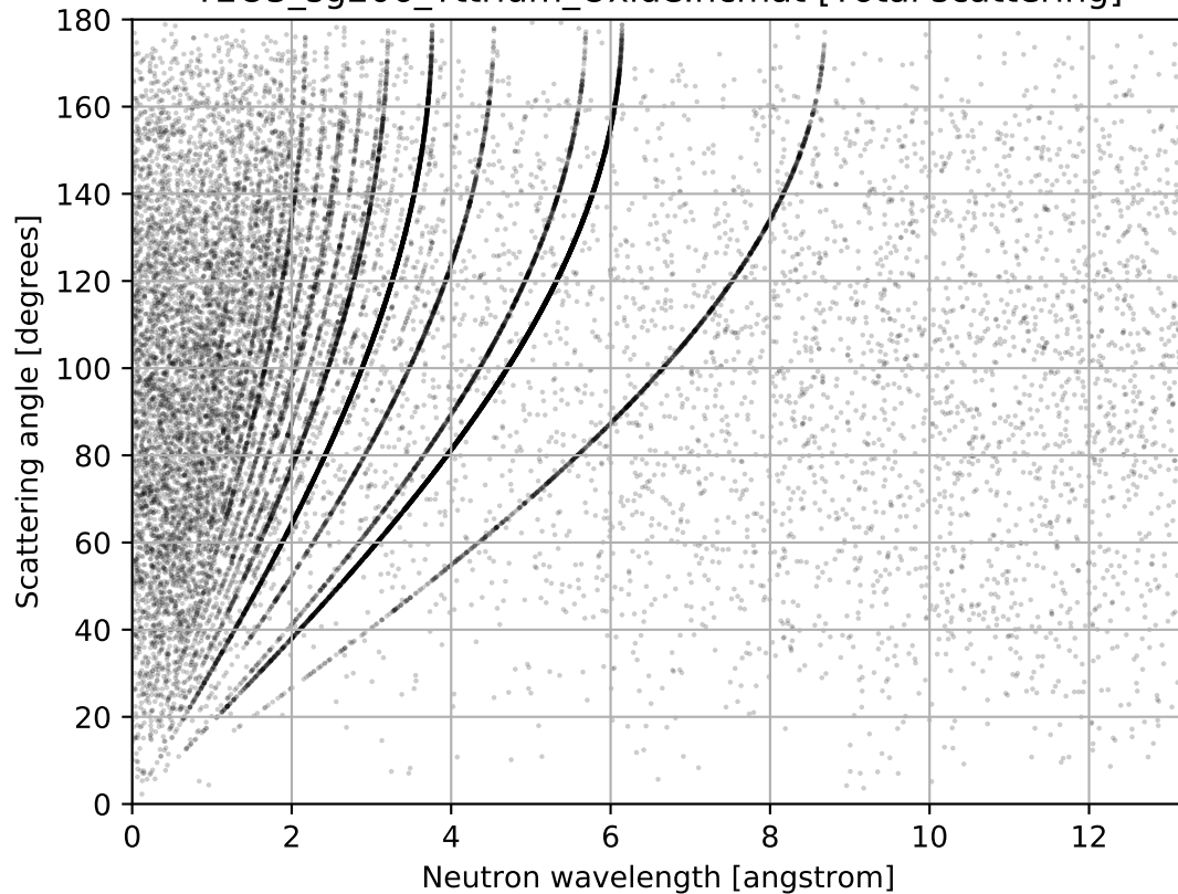
Y2O3_sg206_Yttrium_Oxide.ncmat [Total scattering]
