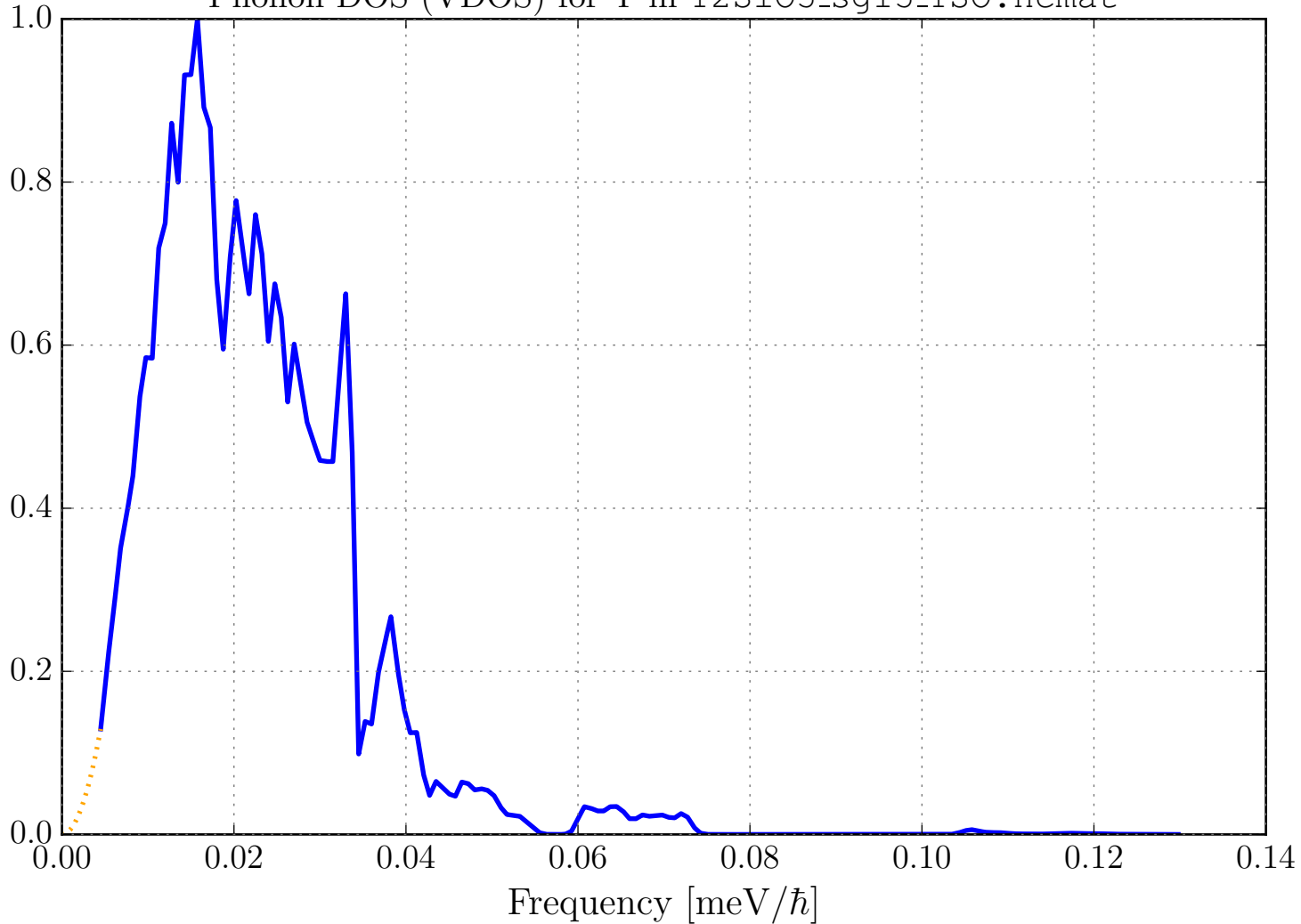
Phonon DOS (VDOS) for Y in Y2SiO5_sg15_YSO.ncmat
