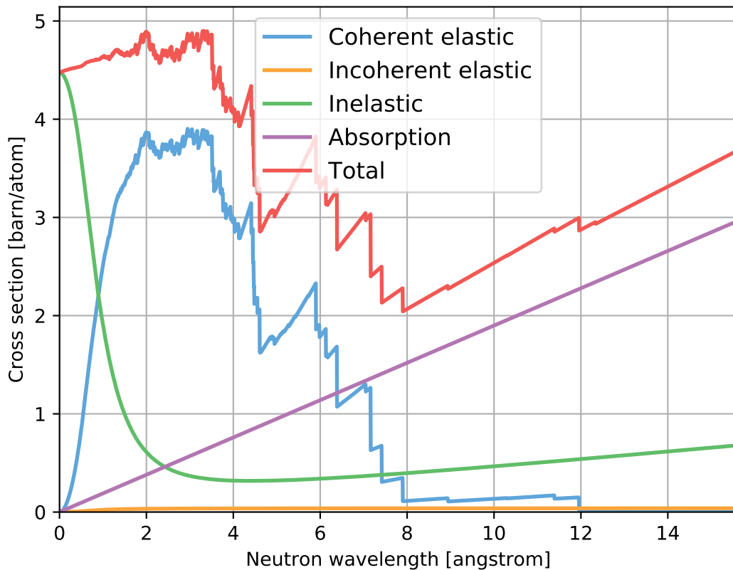
Y2SiO5_sg15_YSO.ncmat [dcutoff=0.3]
