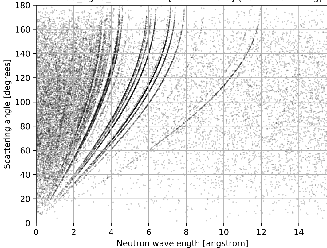
Y2SiO5_sg15_YSO.ncmat [dcutoff=0.3] (Total scattering)
