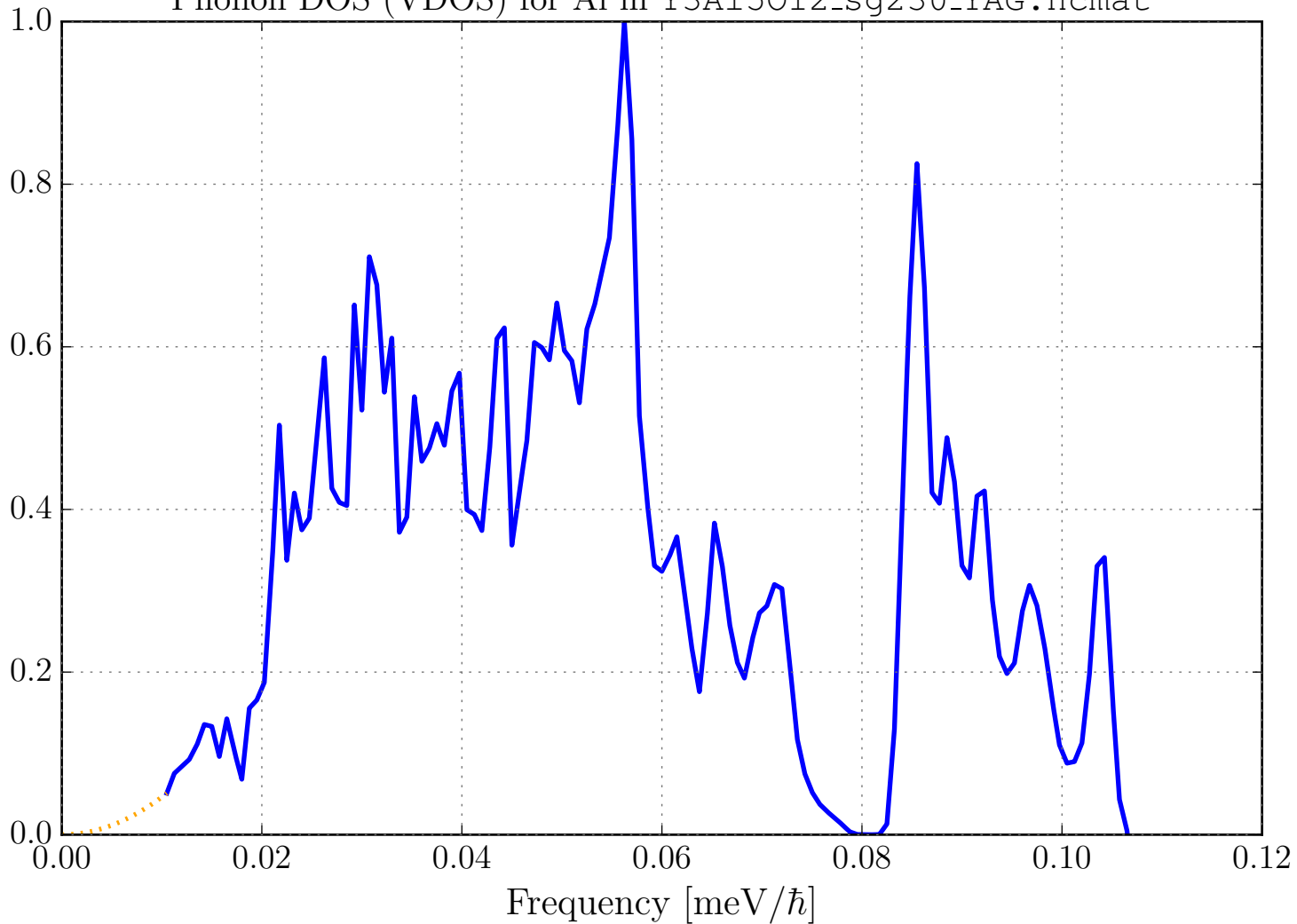
Phonon DOS (VDOS) for Al in Y3Al5O12_sg230_YAG.ncmat
