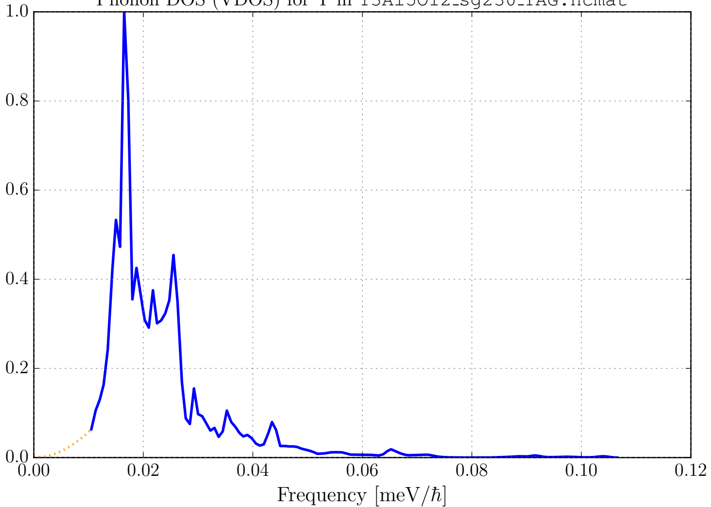
Phonon DOS (VDOS) for Y in Y3Al5O12_sg230_YAG.ncmat
