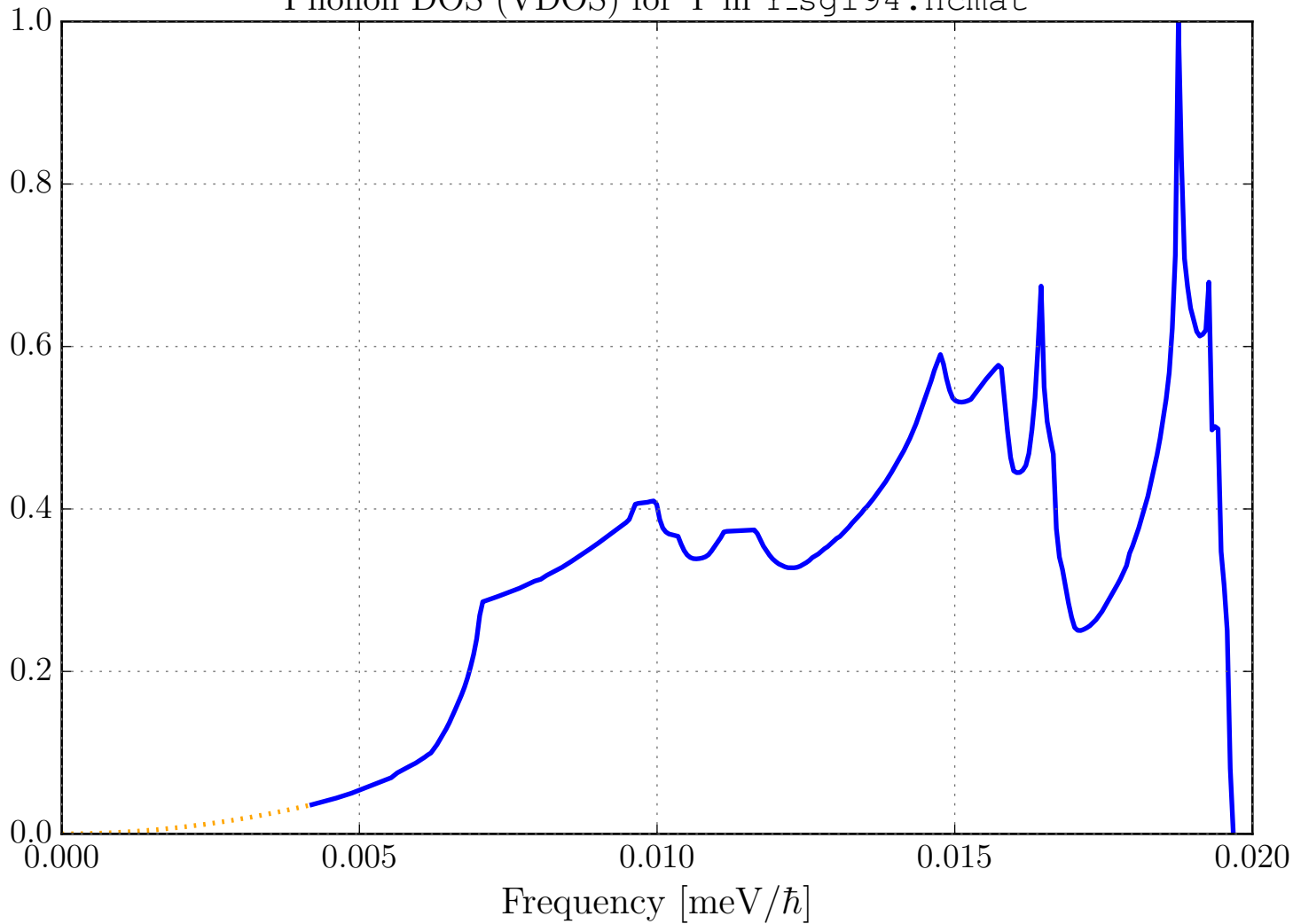
Phonon DOS (VDOS) for Y in Y_sg194.ncmat
