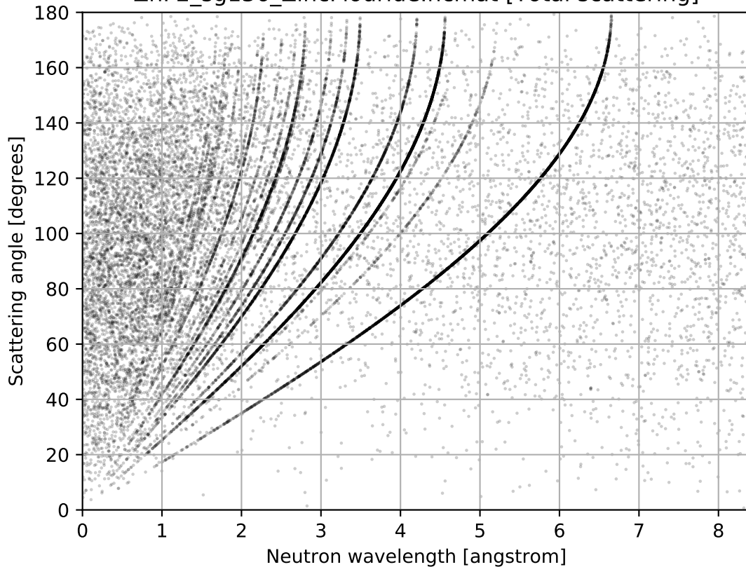
ZnF2_sg136_ZincFluoride.ncmat [Total scattering]
